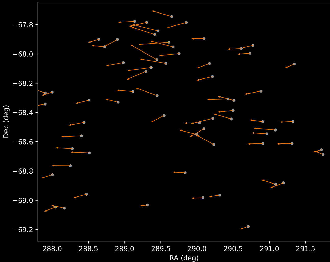
APOGEE DR17 Cluster 2 Proper Motion Vectors (n=66)
