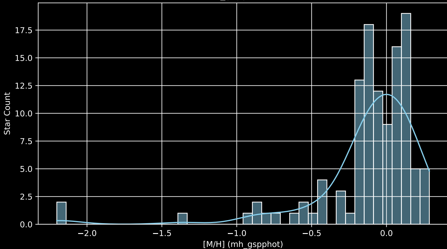
APOGEE DR17 Field: [COL261 [M/H] (mh_gspphot) (n= 117)
