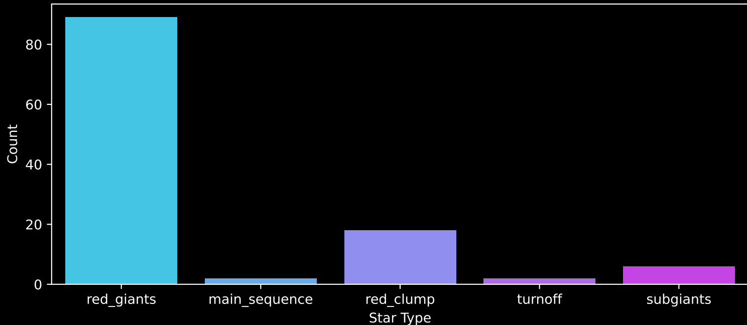
APOGEE DR17 Field: [COL261] Count plot of Star Type
