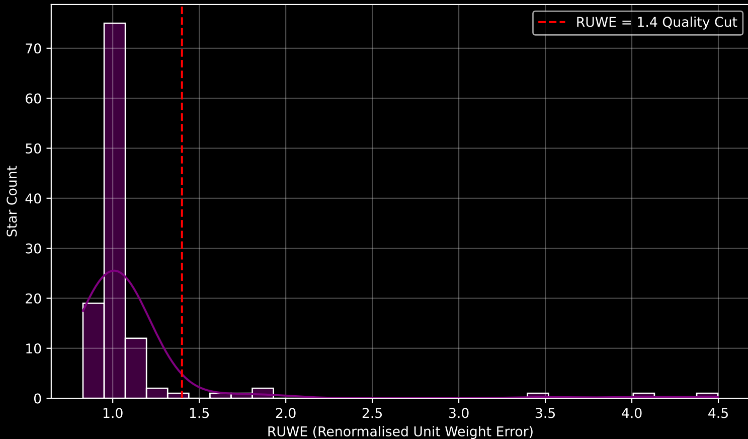
GAPOGEE DR17 Field [COL261] RUWE Distribution (n= 116)
