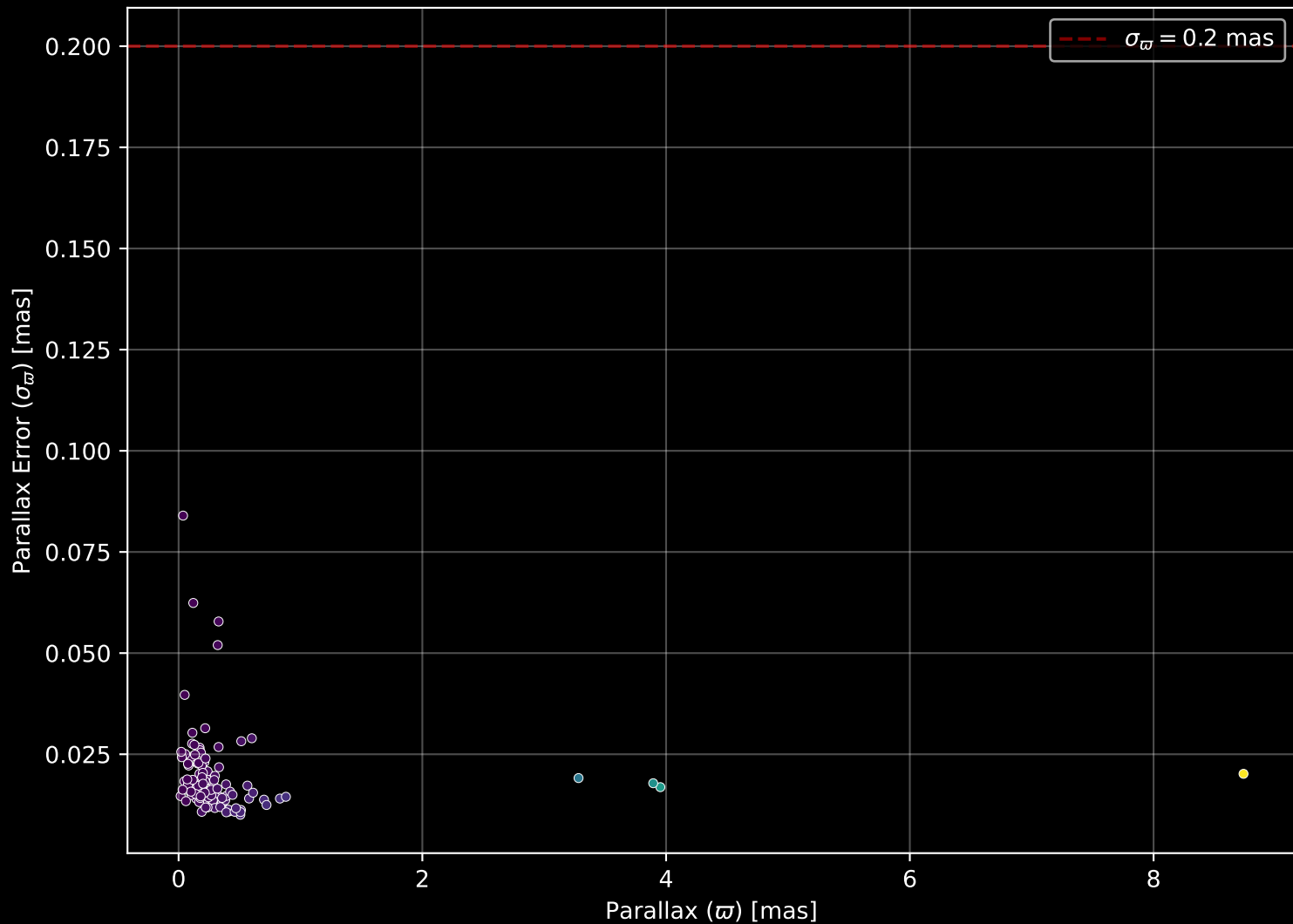
APOGEE DR17 Field: [COL261] Parallax Quality (n= 117)
