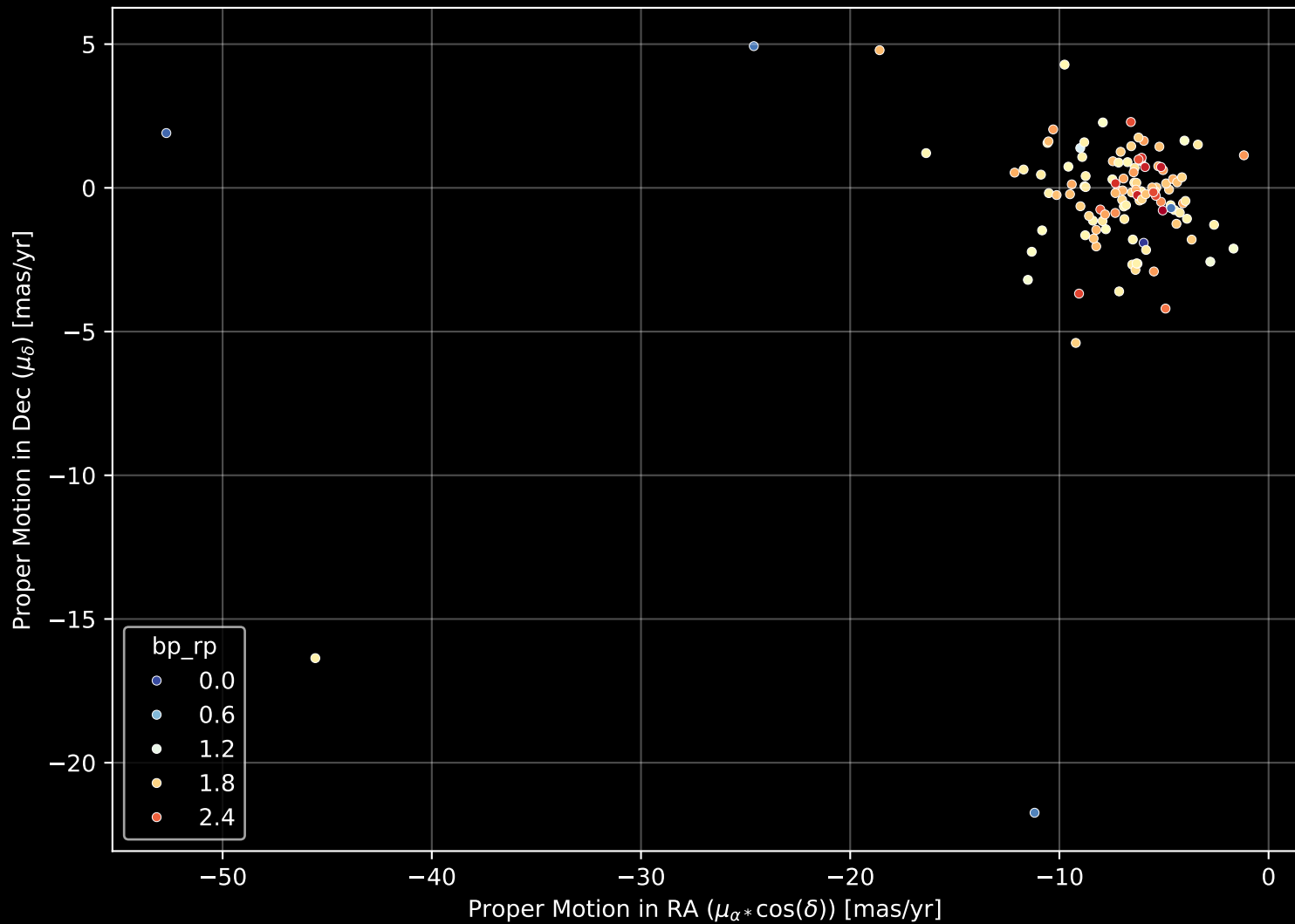
APOGEE DR17 Field: [COL261] Proper Motion Diagram (n= 117)
